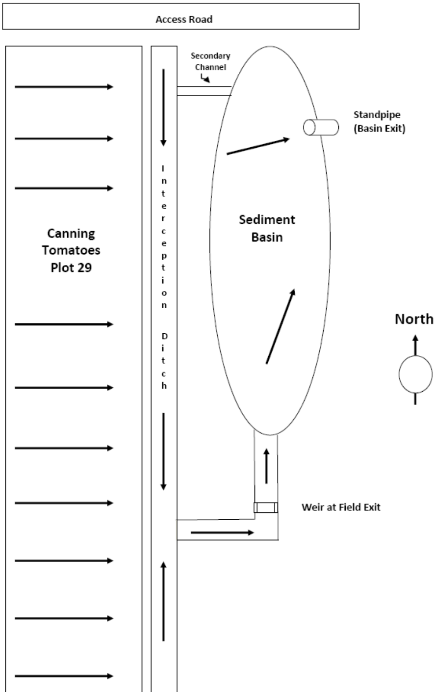
Figure 5. Plot Diagram for Sediment Basin Study
