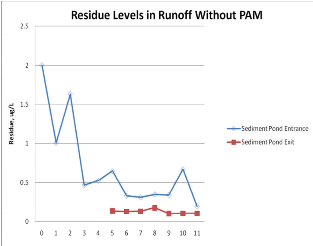
Figure 12. Pyrethroid Residues in Runoff Samples Without PAM Treatment
